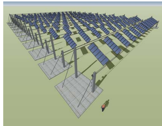
Figure 2: Sketch of Solar Wings mounting system.
