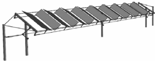
Figure 13: Power Wings is a two axis Solar Wings tracking system completed by an independently tracked mirror system with parallel tracking axis mounted on the same two support cables.[13]
