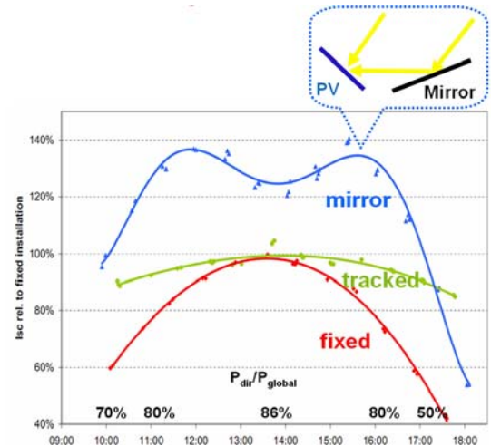
Figure 9: Outdoor measurement results of short-circuit current using the test-setup (Fig. 8) and tracking the PV module assisted by the use of one planar mirror to increase sunlight irradiance. The outdoor measurement was performed in Winterthur on the 2008-08-27 with measured ratio of direct to global irradiance in the horizontal plane of 70% at 10:00, 86% at noon and 50% at 17:00.
