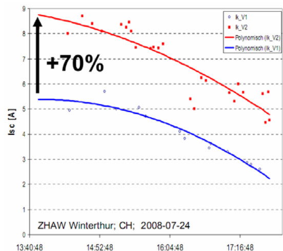
Figure 11: Outdoor measurement results of short-circuit current using the test-setup (Fig. 8) and tracking the PV module assisted by the use of two planar mirrors (Fig. 10) to increase sunlight irradiance. Measurement performed at Winterthur, Switzerland on the 2008-07-24.
