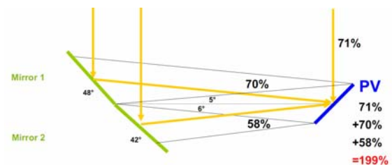
Figure 10: Low-concentration using two planar mirrors.
